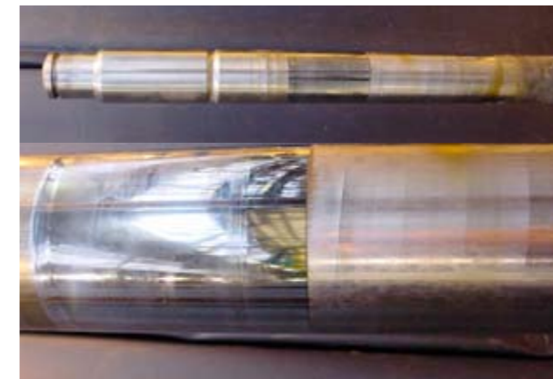
Figure 02: Physical adhesion and abrasive wear of a hard-chromed valve spindle (MC-type after 15,000 hrs)
