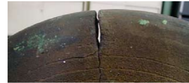
Figure 14: Failure of a valve spindle (RTA84 Nimonic type 5,270 hrs after repair).
