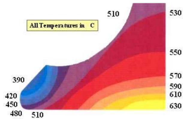
Figure 10: Typical temperature distribution of a Nimonic exhaust valve head
