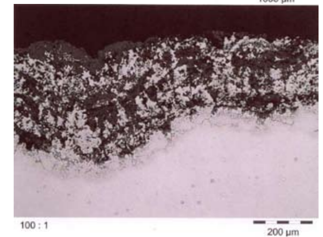
Figure 09: Micro cuts of Nimonic with high-temperature corrosion.
