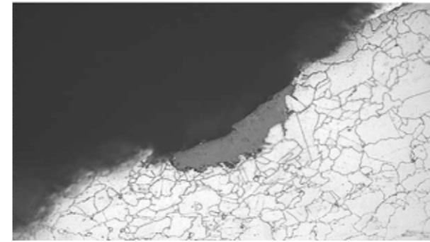
Figure 07: Low temperature corrosion (pitting corrosion attack) of under head radius of valve spindle (MC60-standard / 22,700 hrs)
