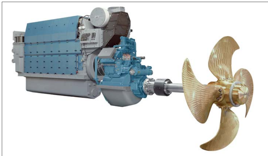
Fig 3. MAN Diesel L27/38 – the complete propulsion solution
